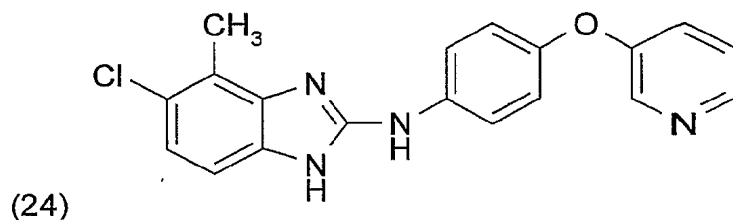
(5-Chlor-4-methyl-1H-benzimidazol-2-yl)-[4-(pyridin-3-yloxy)-phenyl]-amin
